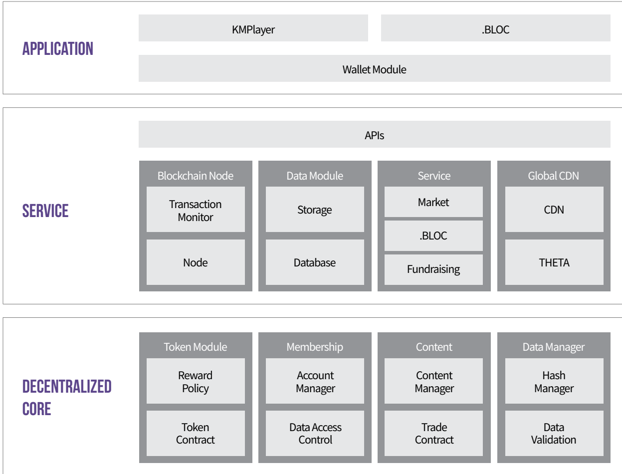
Fig. 10. MovieBloc Architecture
