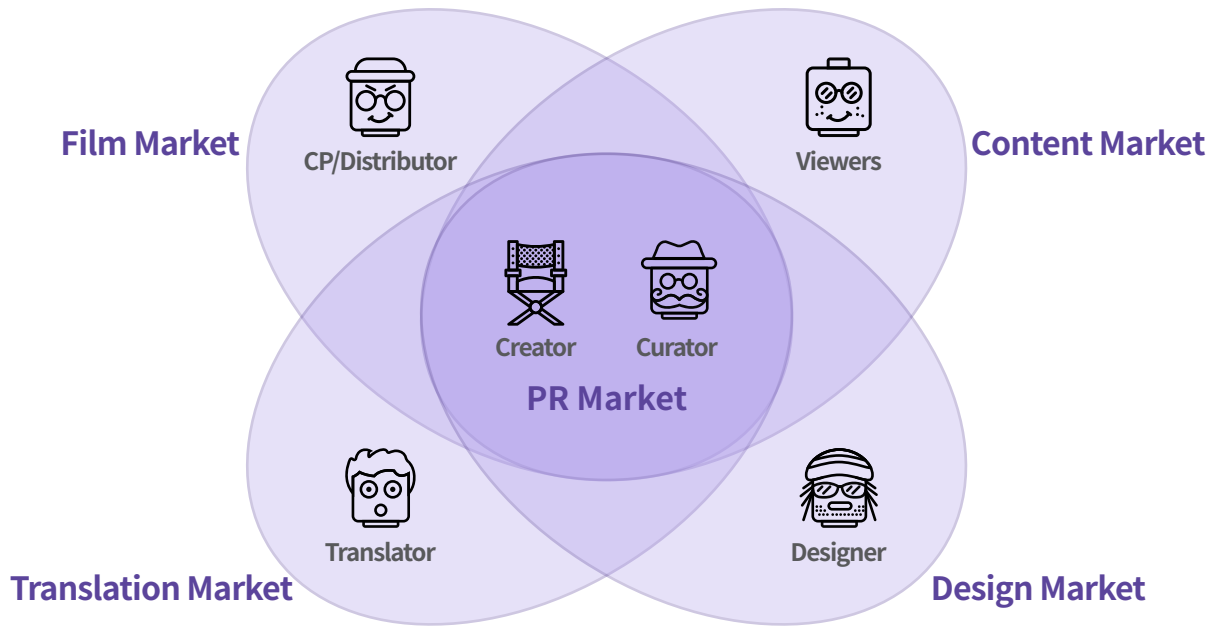
Fig. 8. MovieBloc Market
