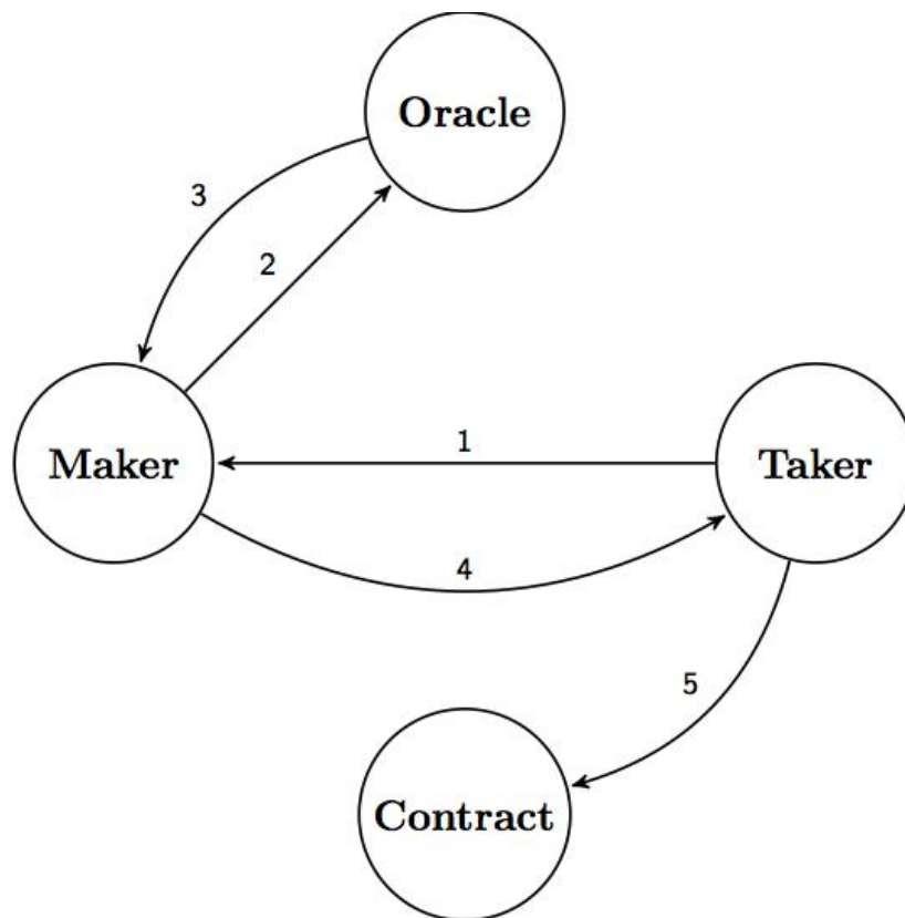
Figure 5: Maker querying Oracle before providing order
