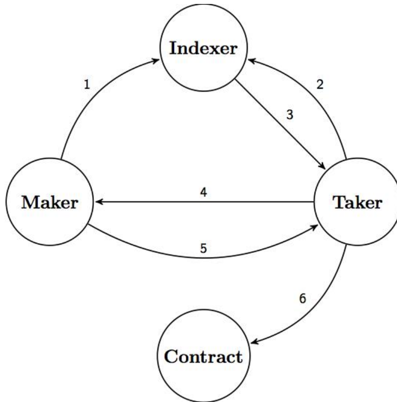
Figure 2: Find a counterparty and make a trade
