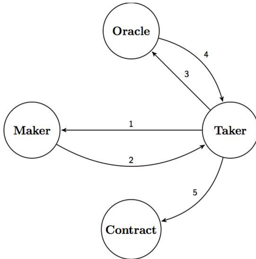
Figure 6: Taker querying Oracle before filling order
