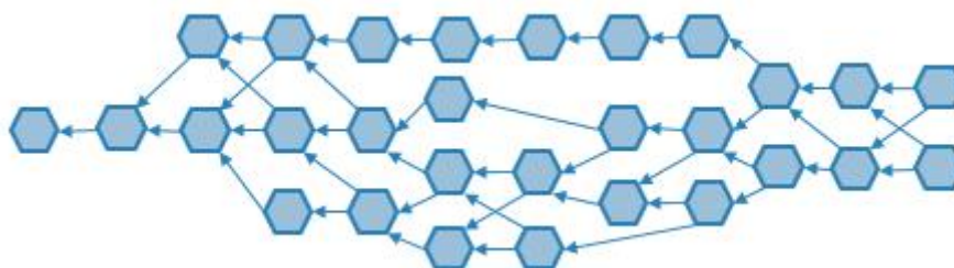
Figure 2-1 DAG Graph
