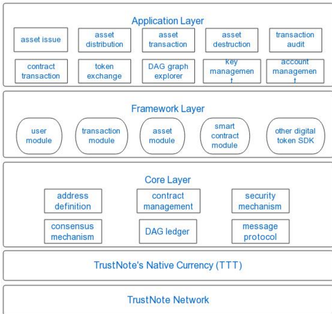
Figure 6-2 Architecture of Crypto-Token Platform
