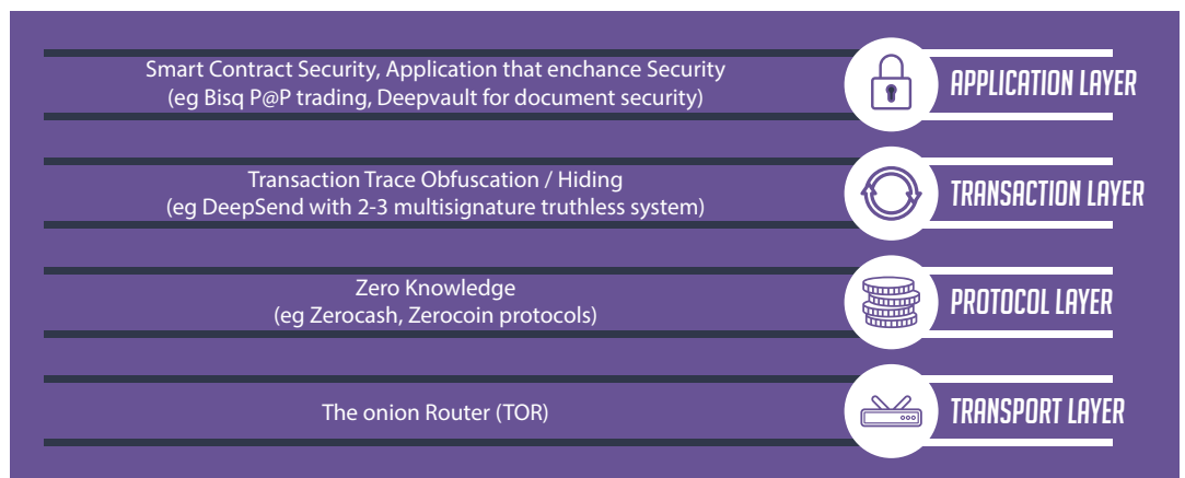
Fig. 1 DeepOnion's Multi-layered Security Model
